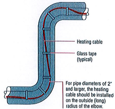
Figure 15: Elbow
