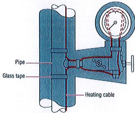
Figure 12: Pressure gauge
